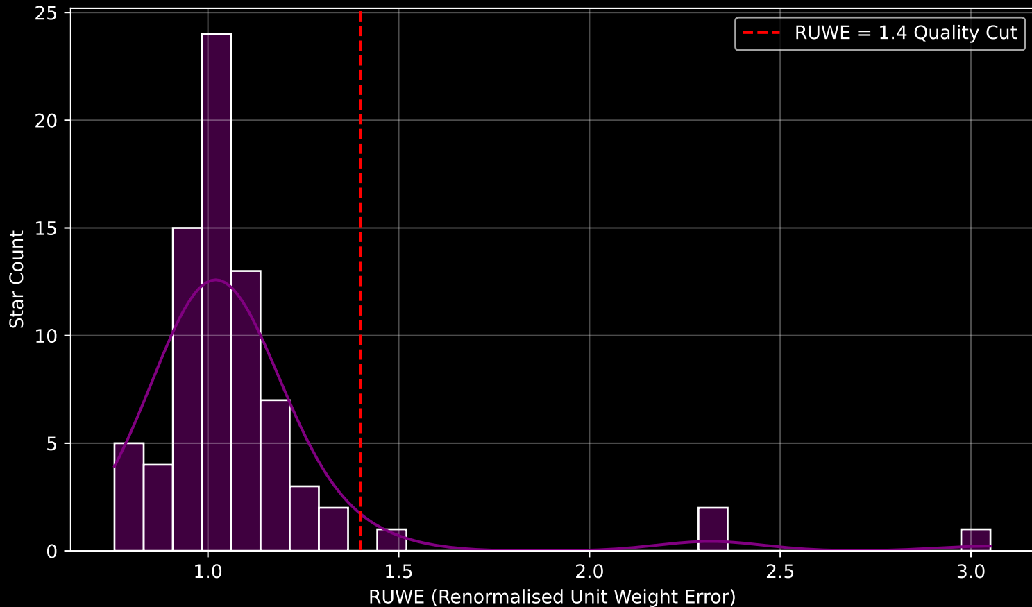
GAPOGEE DR17 Field [302-43-O] RUWE Distribution (n= 77)
