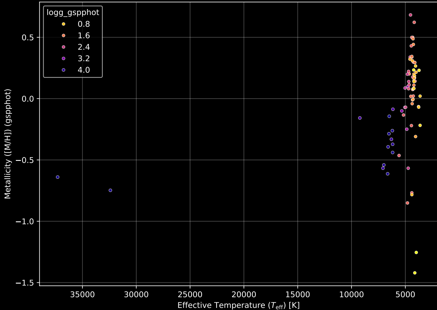
APOGEE DR17 Field: [302-43-O] Stellar Population Parameters (n= 78)
