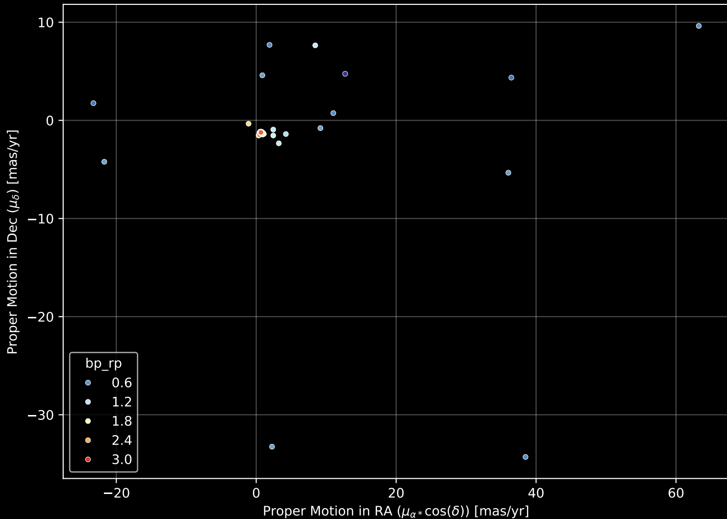
APOGEE DR17 Field: [302-43-O] Proper Motion Diagram (n= 78)
