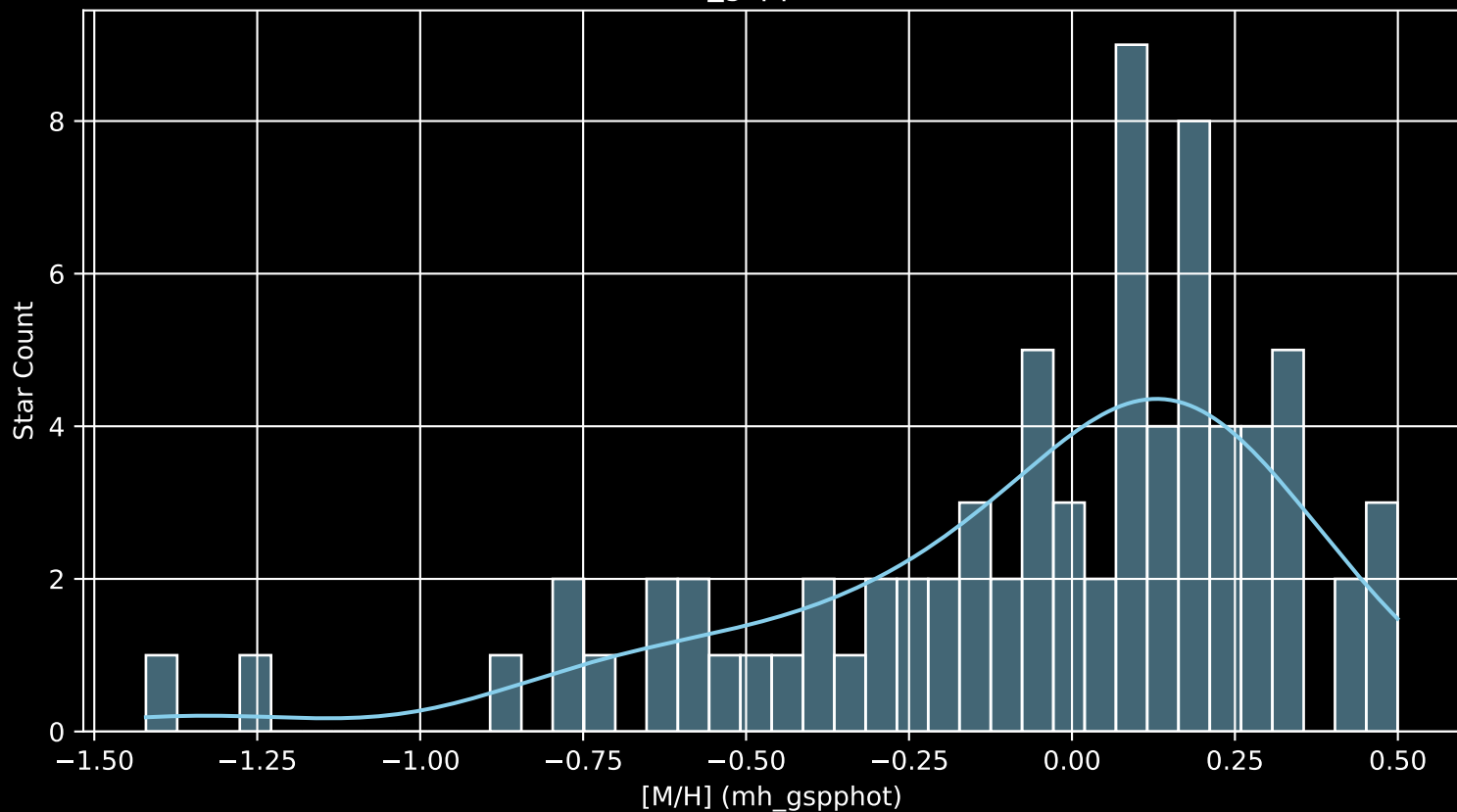
APOGEE DR17 Field: [302-43-O [M/H] (mh_gspphot) (n= 76)
