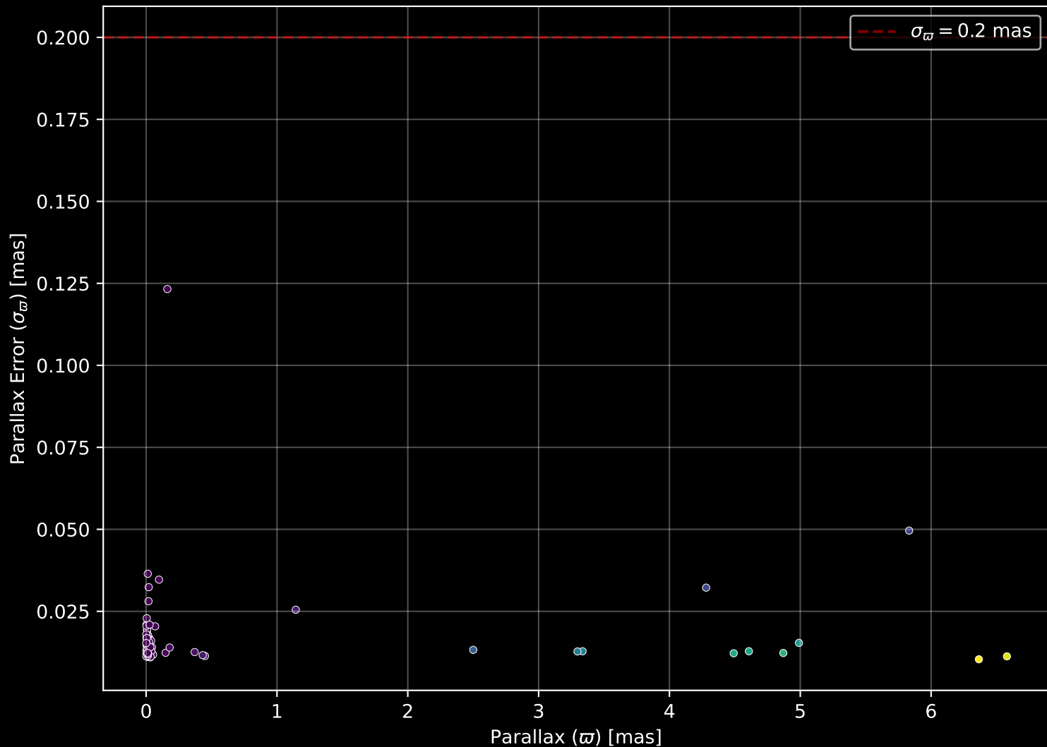
APOGEE DR17 Field: [302-43-O] Parallax Quality (n= 78)
