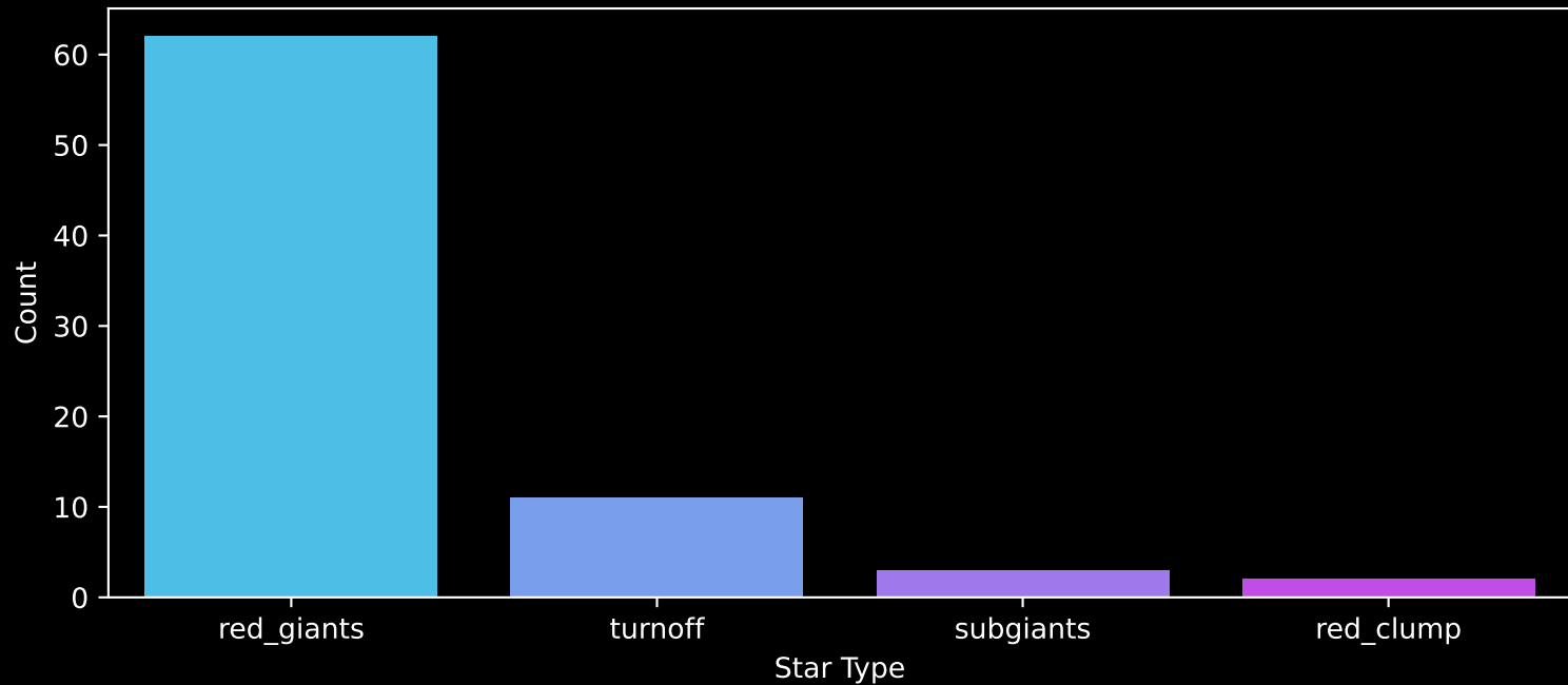
APOGEE DR17 Field: [302-43-O] Count plot of Star Type
